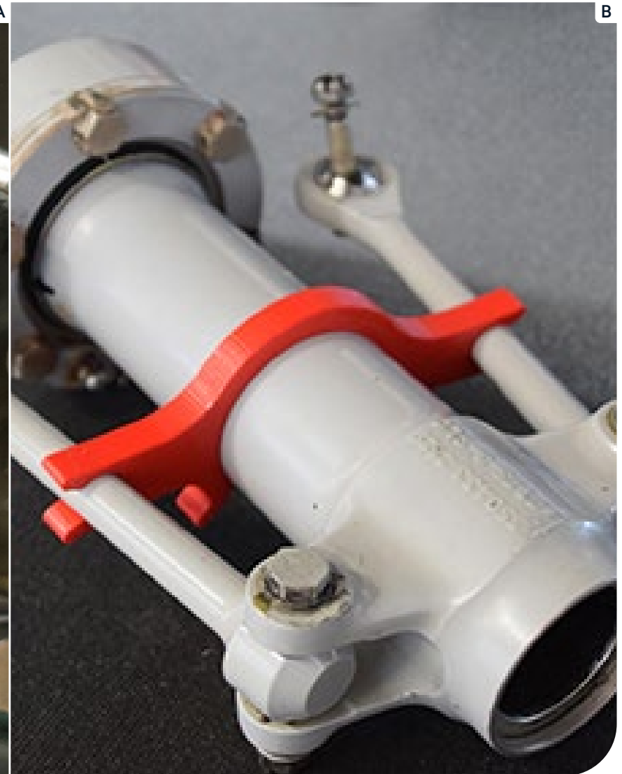
A Torque Transmitter | B TR PCL Holder
